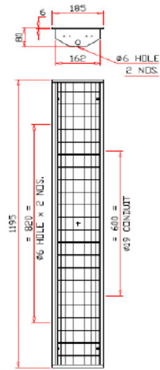
Nominal Dimensions in mm, Tolerance +/- 2 mm
